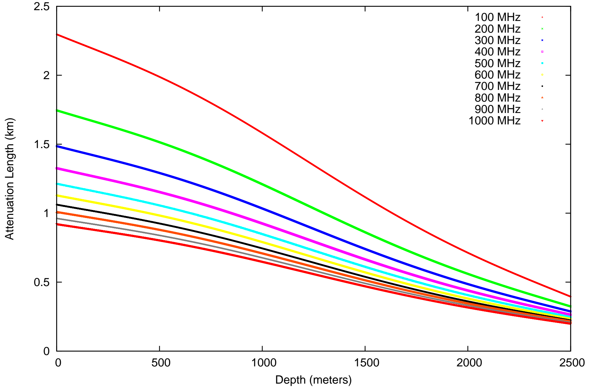
Bogorodsky Ice Attenuation Versus Temp And Frequency Model
