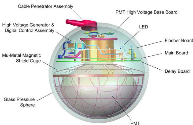
Fig.2: Digital optical modules (DOMs) are pressure resistant glass spheres, each containing a Hamamatsu photomultiplier tube (PMT) of 25 cm diameter and the associated electronics necessary for waveform digitization [12][13].
