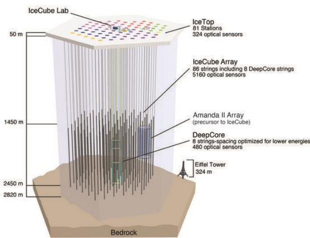
Fig.1: The IceCube Neutrino Observatory instruments roughly one cubic kilometer of clear Antarctic ice with 86 strings anchored at depth of about 2450m and each containing 60 digital optical modules (DOMs).
