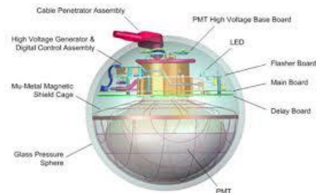
Fig.2: Digital optical modules (DOMs) are spherical, pressure resistant glass spheres, each containing a Hamamatsu photomultiplier tube (PMT) of 25 cm diameter and the associated electronics necessary for waveform digitization [5,6].
