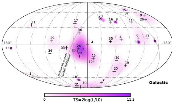
Fig.4: Skymap in galactic coordinates using the highest energy neutrino event sample arrival directions.
