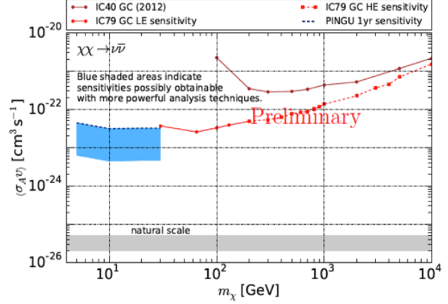
Fig.7: Sensitivity with one year of PINGU data to the spin-dependent WIMP-proton scattering (left) and dark matter annihilating in the Galactic center (right) [28].
