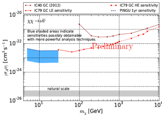
Fig.7: Sensitivity with one year of PINGU data to dark matter annihilating in the Galactic center [37].
