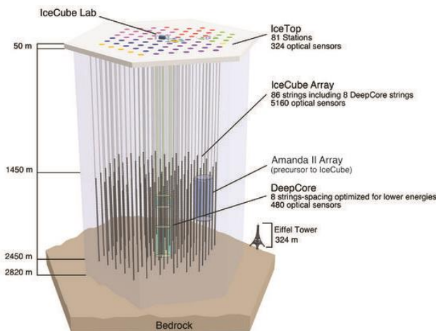
Fig.1: The IceCube Neutrino Observatory instruments a volume of roughly one cubic kilometer of clear Antarctic ice with 86 strings anchored at depth of about 2450m and each containing 60 digital optical modules (DOMs). The observatory includes a densely instrumented subdetector, DeepCore, and a surface air shower array, IceTop.
