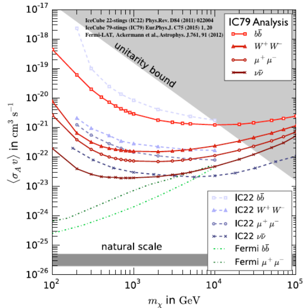
Fig.5: Limit on the dark matter self-annihilation cross section are shown [20, 21]. The natural scale assumes dark matter is a thermal relic of the early Universe [nat].
