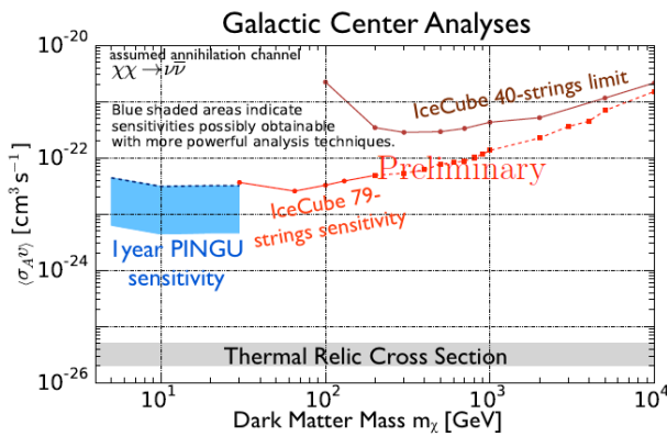
Fig.7: Sensitivity with one year of PINGU data to dark matter annihilating in the Galactic center [37].
