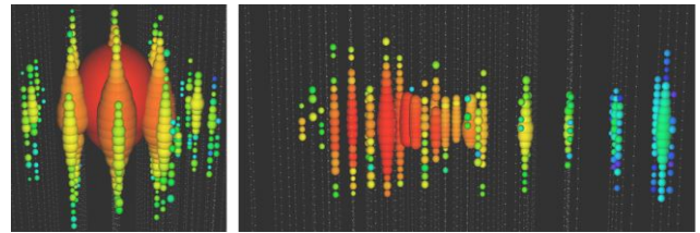
Fig.3: Left: The most energetic neutrino event observed with energy of about 2 PeV [11]. This event nicknamed “Big Bird” shows a spherical topology as expected from an electron neutrino interaction. Right: A track-like event, the typical signature of a detected muon neutrino. Colors indicate the time and the diameter of each sphere represents the number of photons detected by the corresponding DOM.
