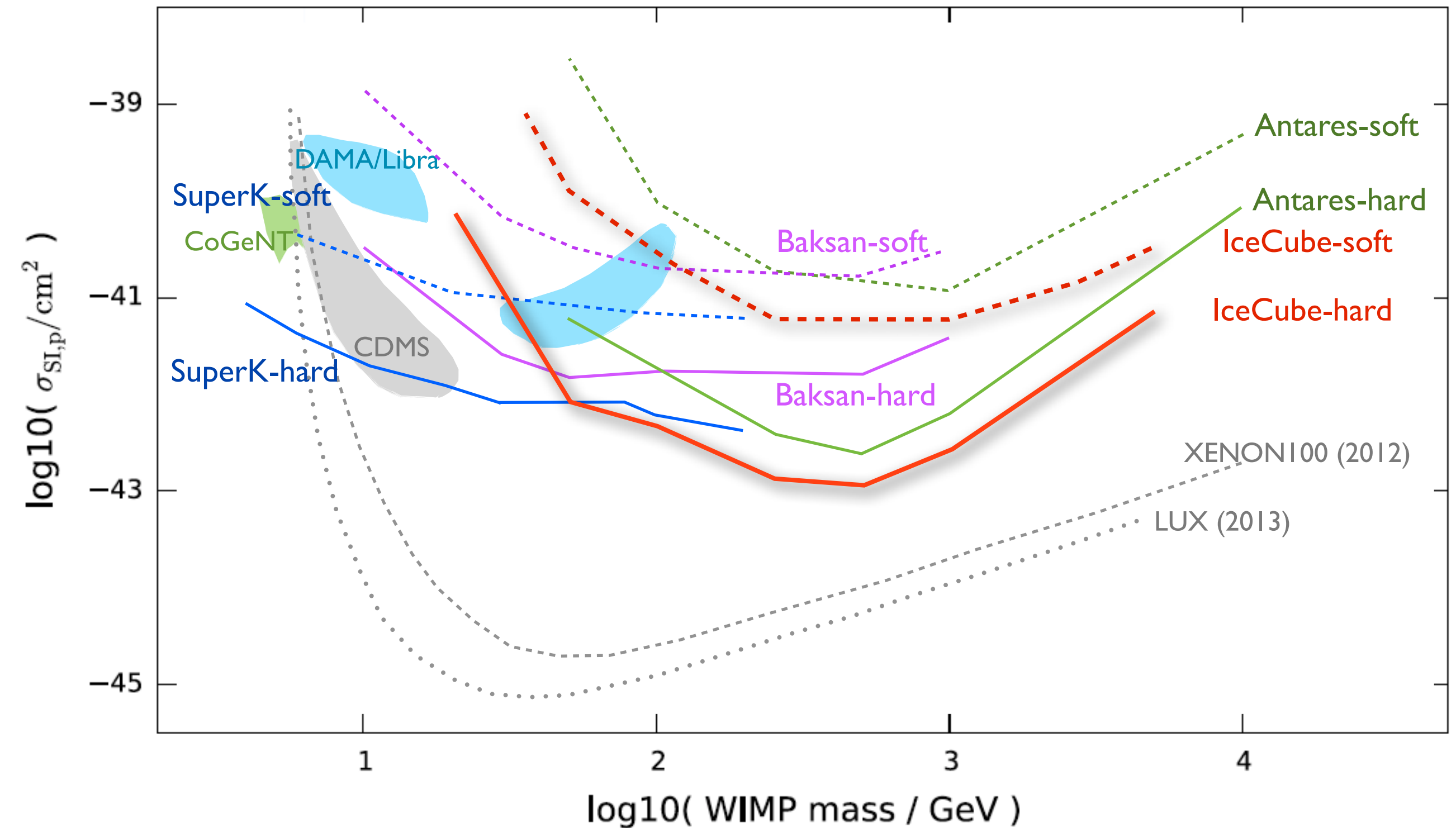
Spin independent WIMP-nucleon cross section
