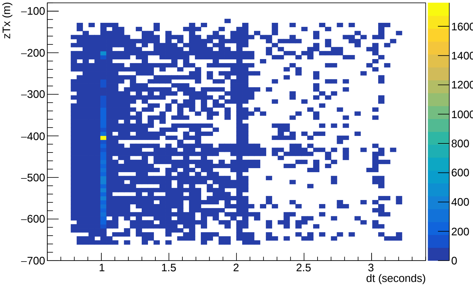
dt(Successive evt triggers, loose evt cuts) as f(z_{Tx})
