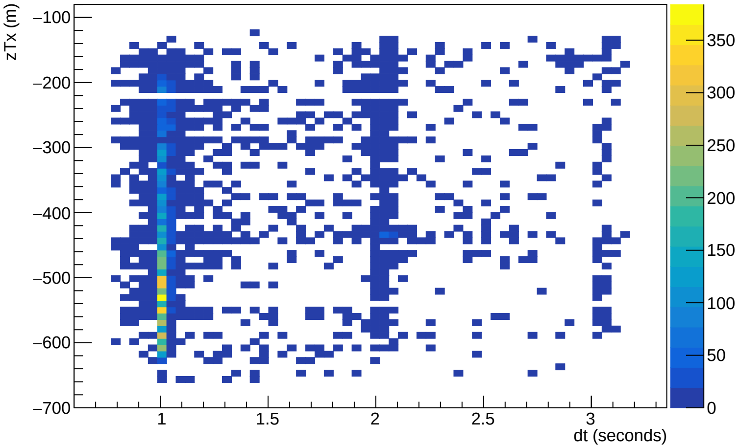
dt(Successive evt triggers, tight evt cuts) as f(zTx)
