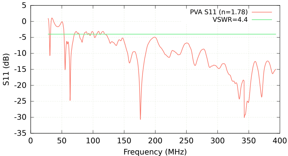
PVA Reflection Coefficient
