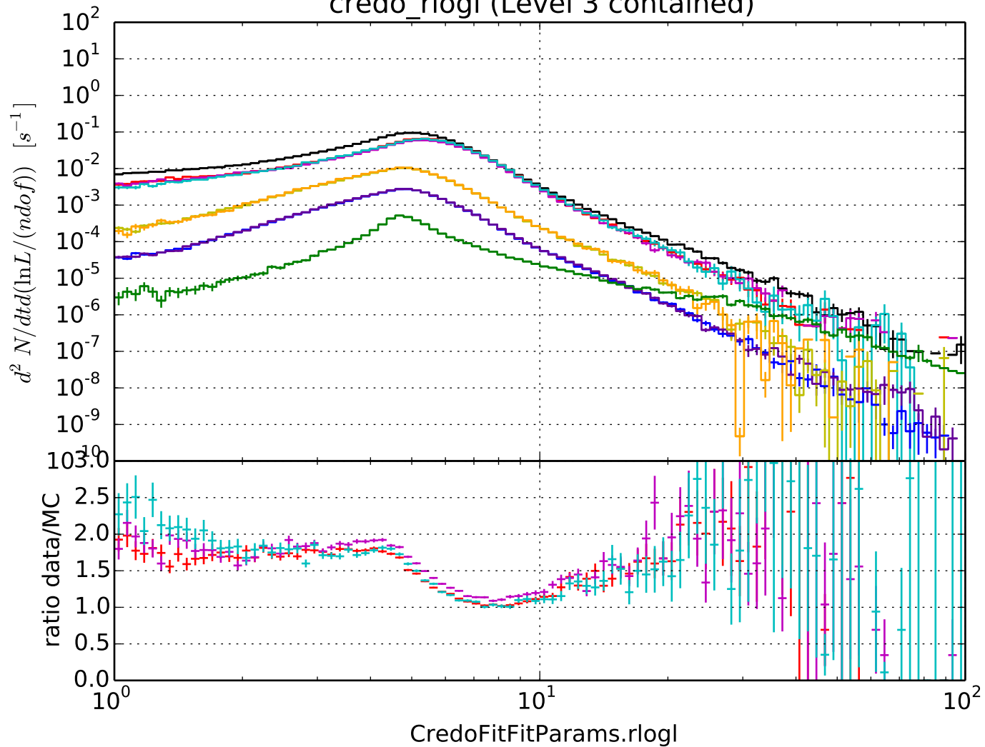
credo_rlogl (Level 3 contained)
