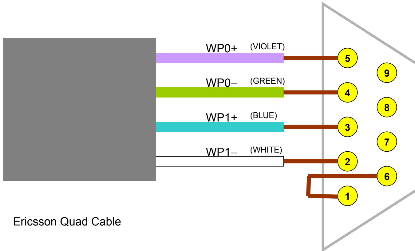
DB-9 Male Connector
