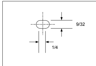
19" Panel Mounting Hole Detail
