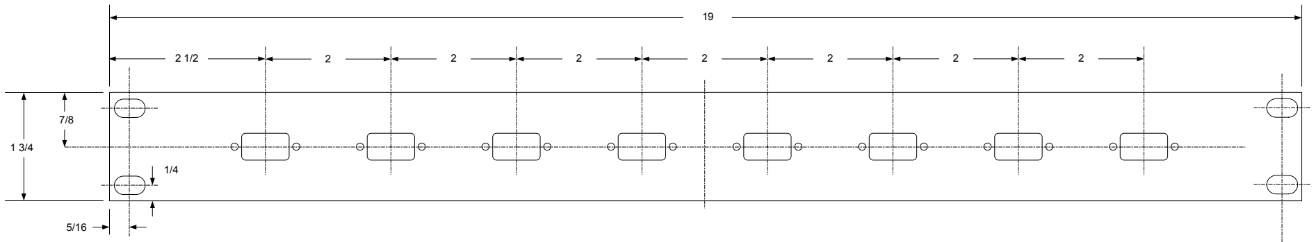
D-Sub Connector Mounting Hole Detail
