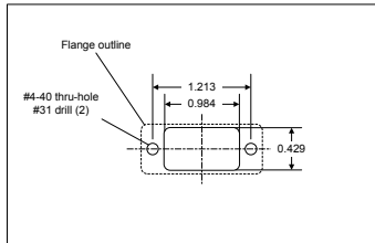
D-Sub Connector Mounting Hole Detail
