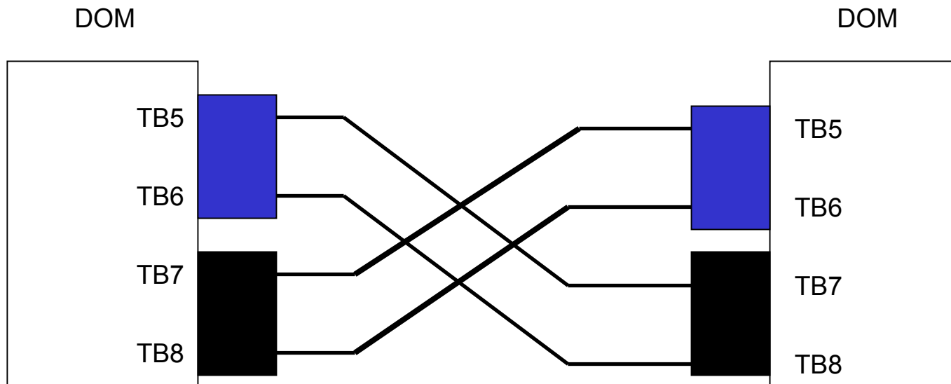
Local Coincidence Connections (according to Jerry Przybylski email, 10/6/2003)
