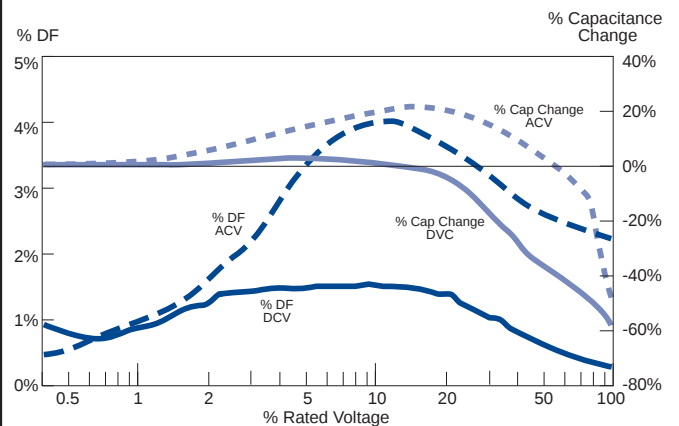
FIGURE 8. Z5U Capacitance & DF versus Applied AC/DC Voltages
