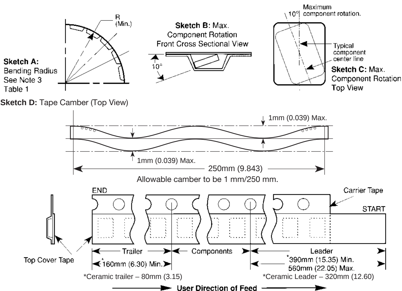
Figure 2: Tape Leader & Trailer Dimensions (Metric Dimensions Will Govern)
