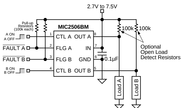
Single and Dual Switch/Circuit Breakers with Open-Load Detection and Fault Output
