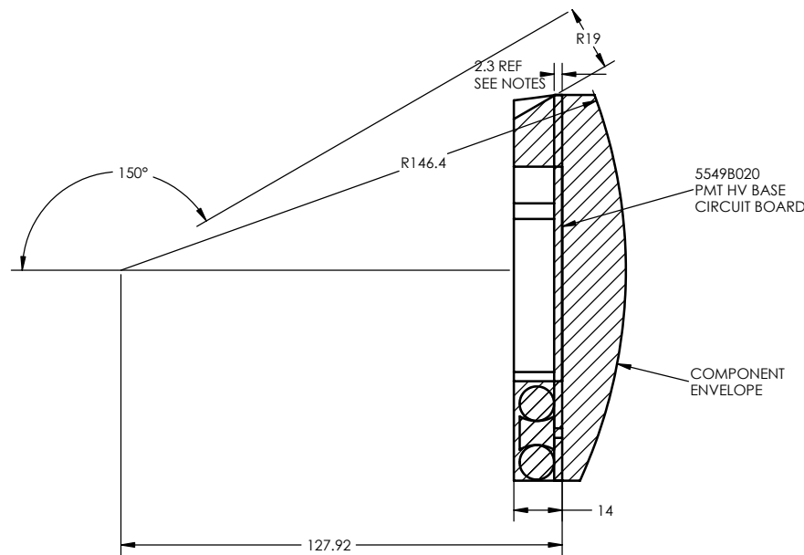
SECTION B-B
