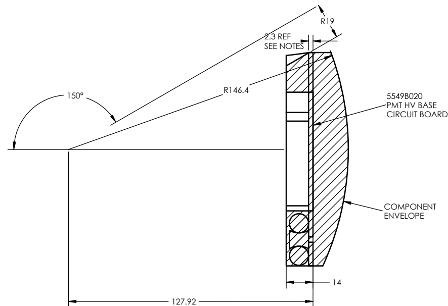
SECTION B-B
