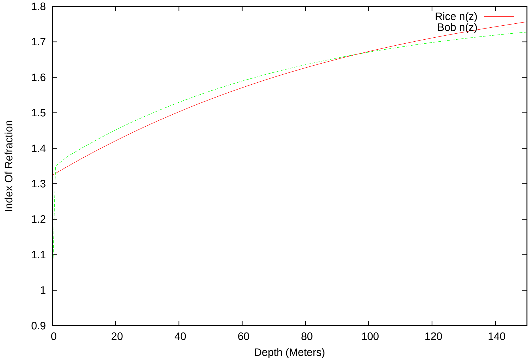
Index Of Refraction Versus Depth
