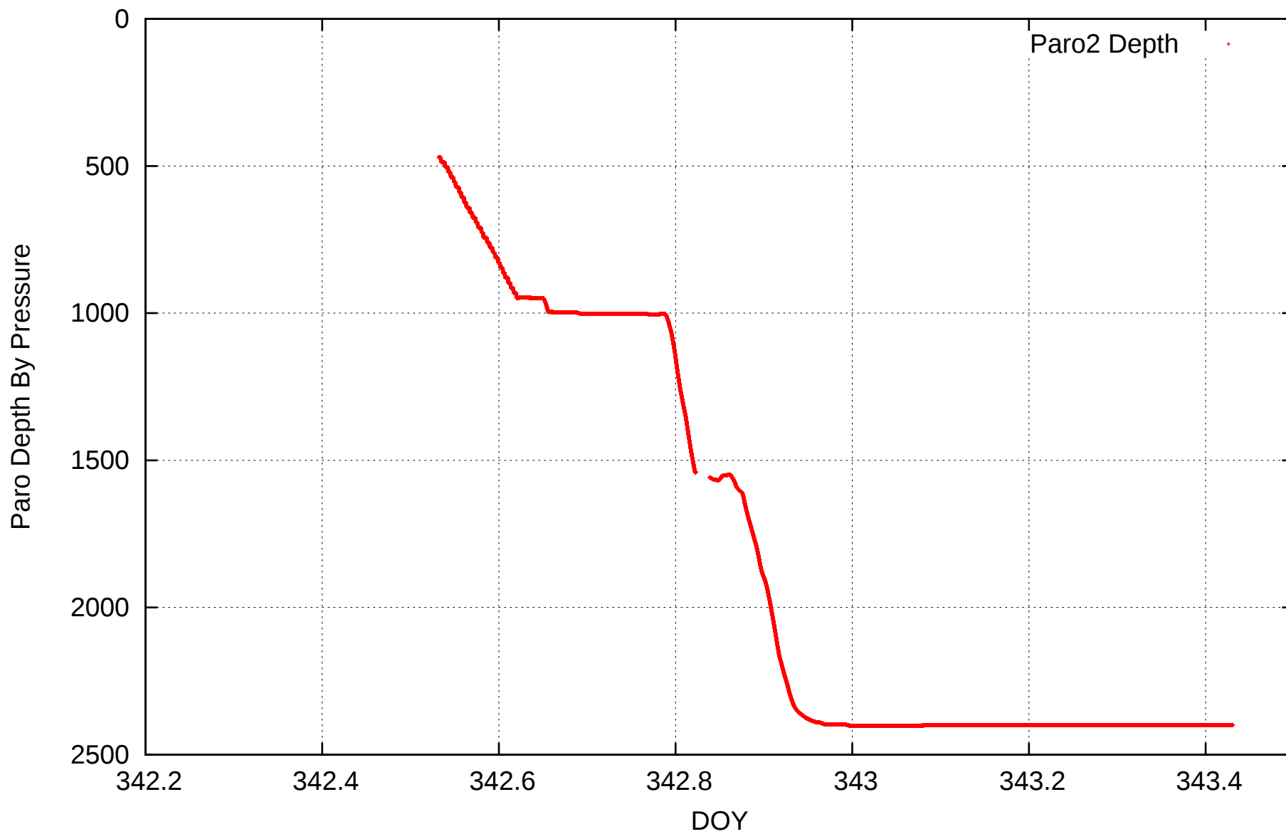
Paro Depth By Pressure Vs. Time From 12/8/2010 4:48:00 to 12/9/2010 12:00:00
