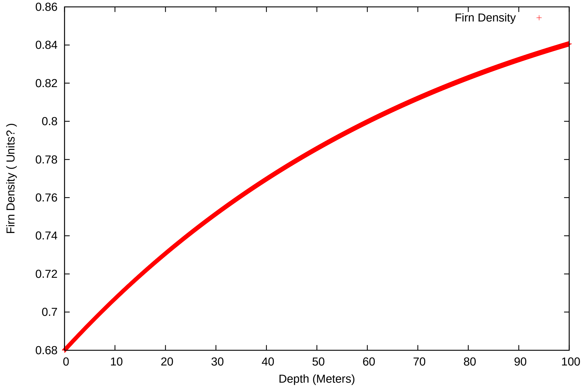
Firn Density Versus Depth
