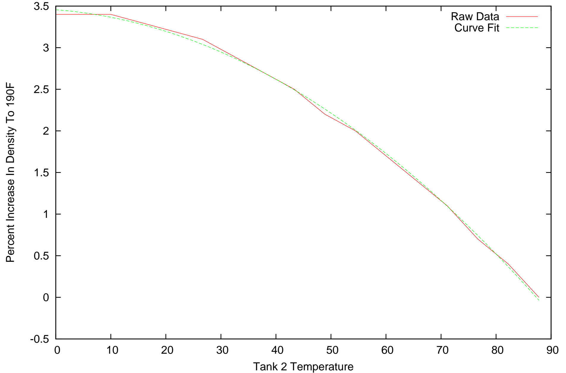
Percent Density Change When Water Heated To 190F
