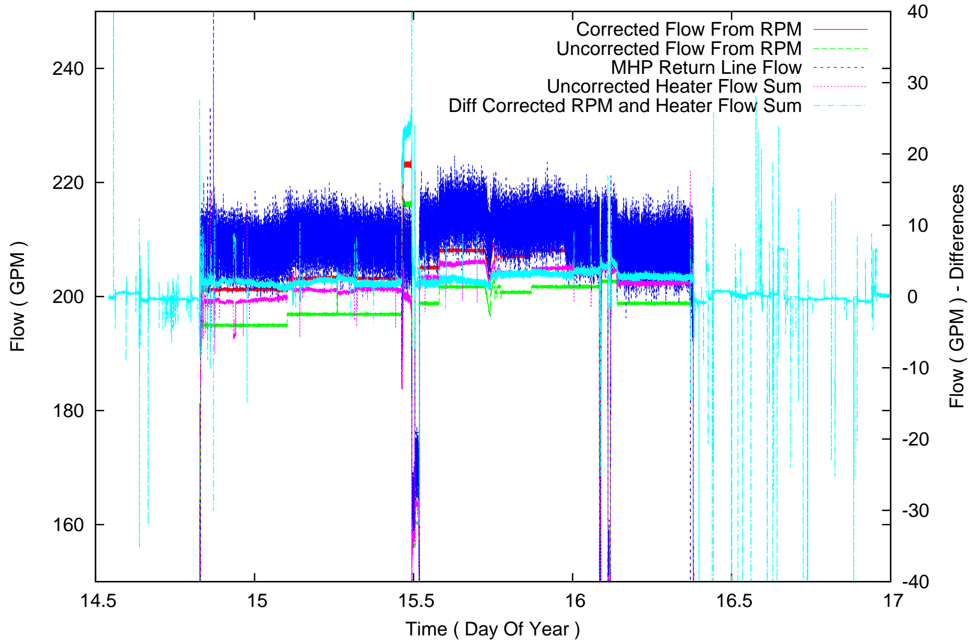
db.Hole48.mnewcomb - Flows
