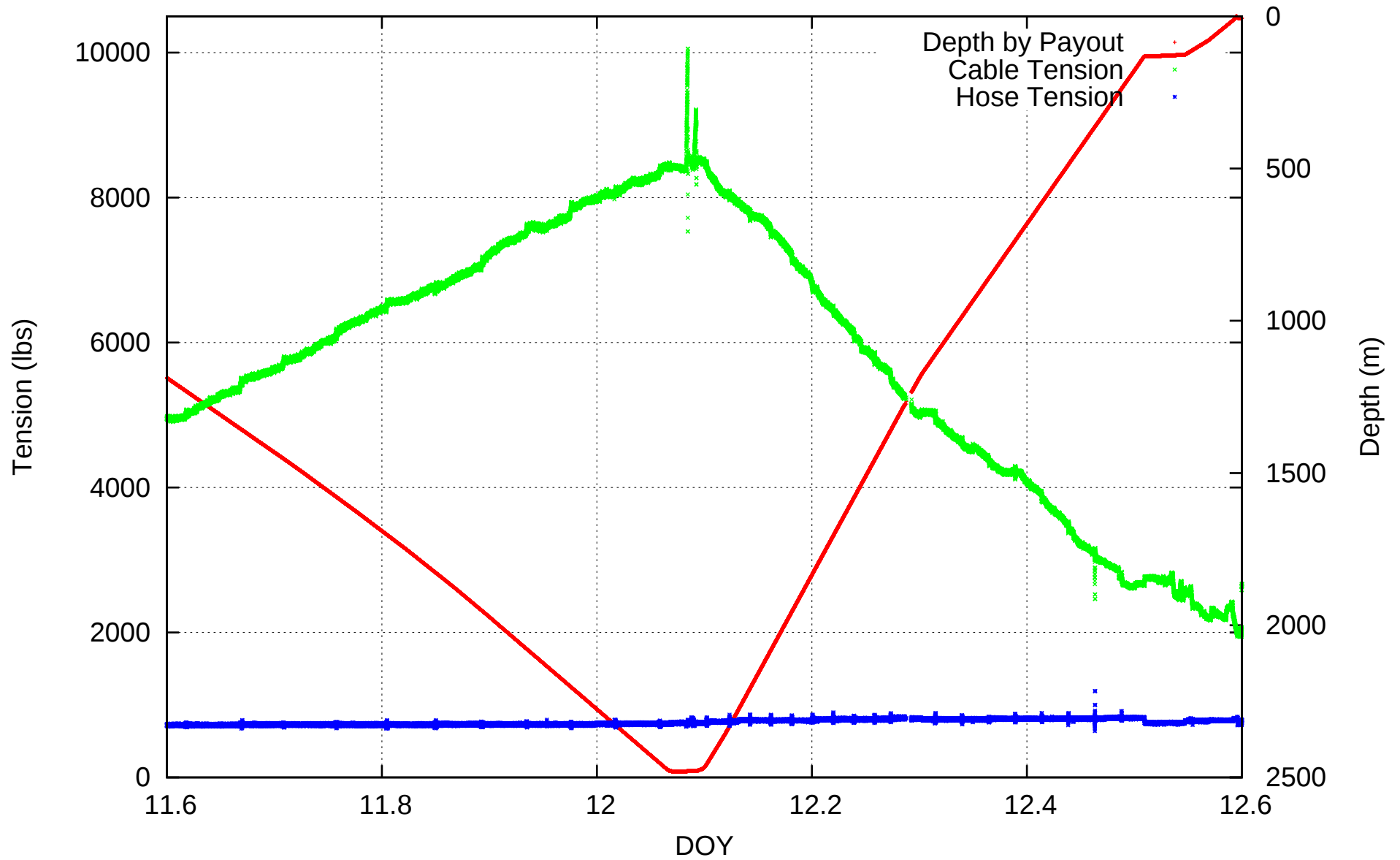
Depth And Load Vs. Time From 1/11/2008 0:00:00 to 1/12/2008 14:24:00
