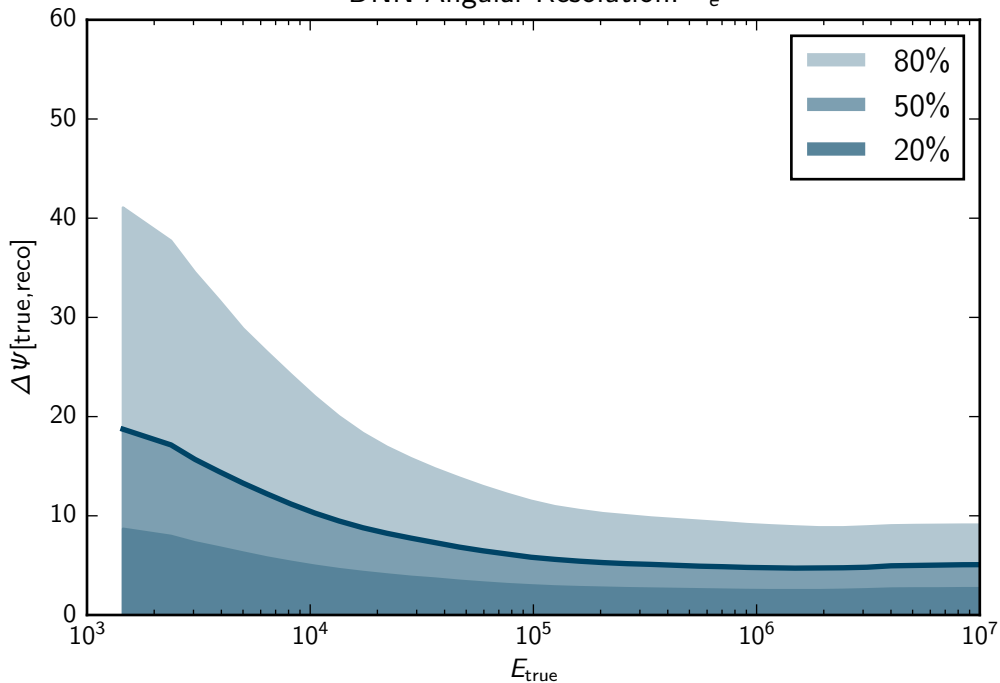
DNN Angular Resolution: e
