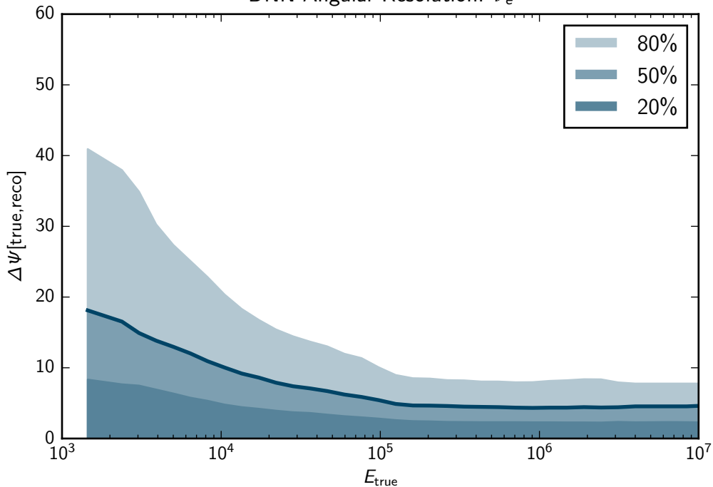
DNN Angular Resolution: \nu_e
