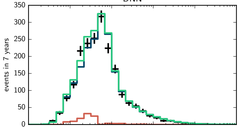
DNN
