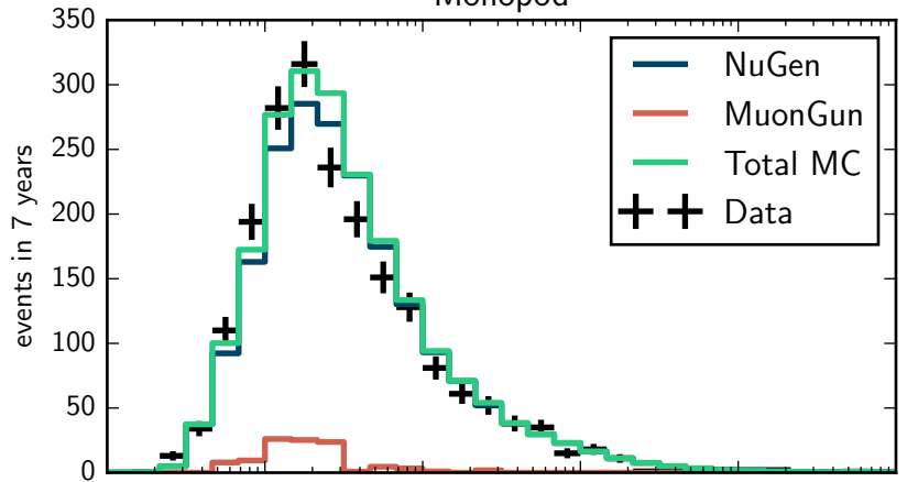
Monopod
