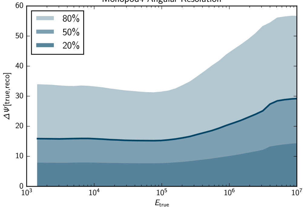
Monopod4 Angular Resolution
