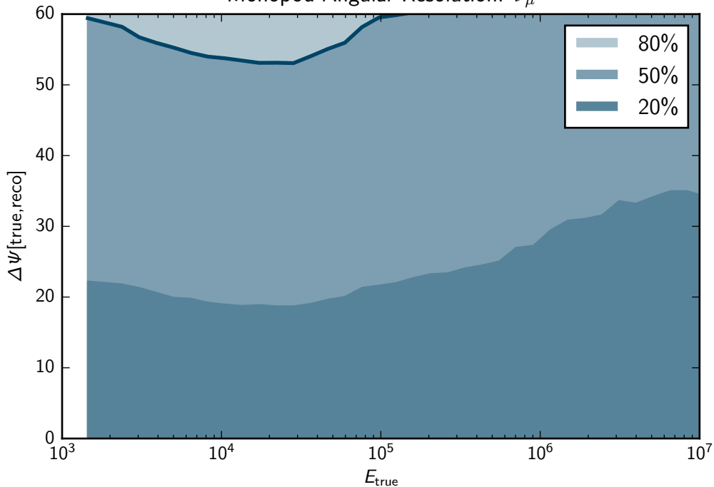
Monopod Angular Resolution: \nu_\mu
