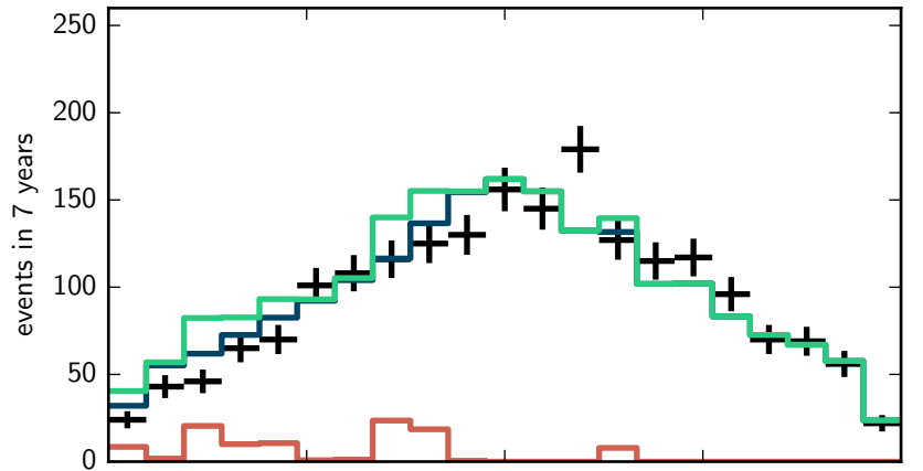
DNN
