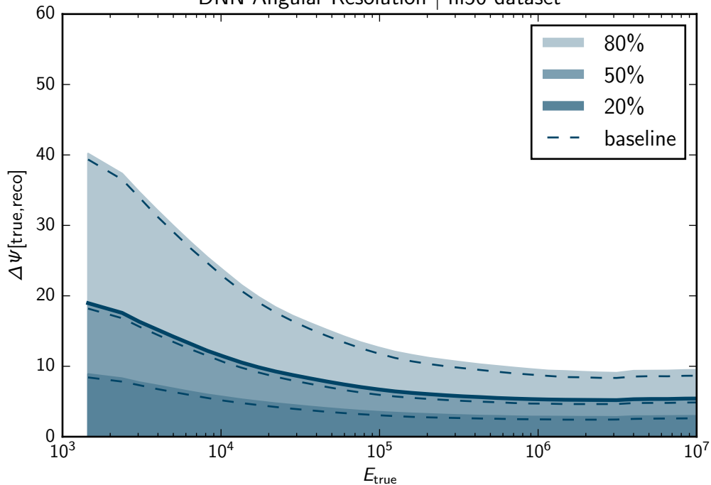
DNN Angular Resolution | hi50 dataset
