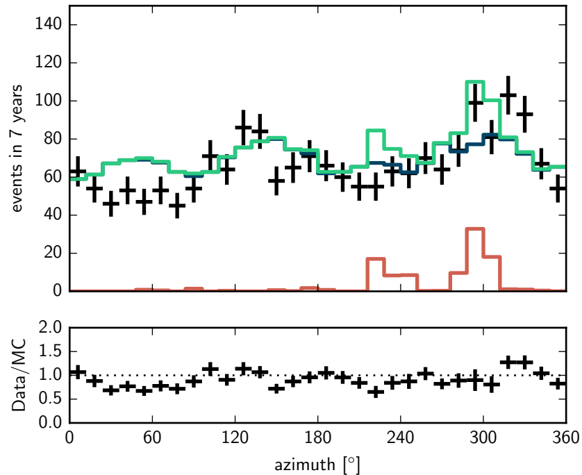
DNN
