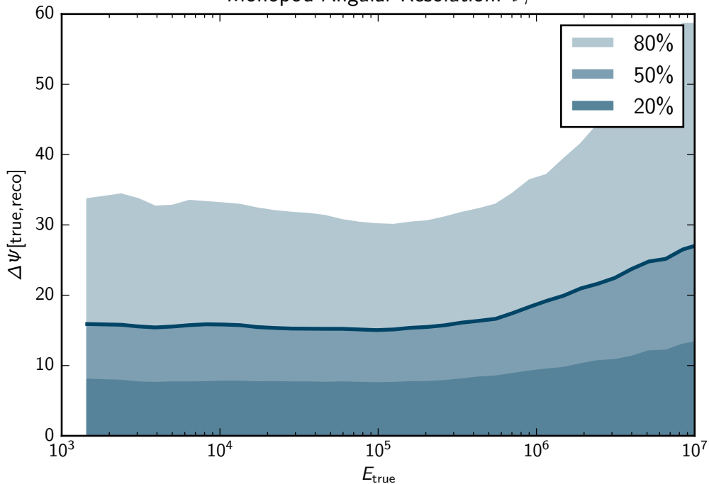
Monopod Angular Resolution: \nu_\tau
