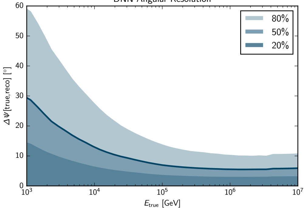
DNN Angular Resolution
