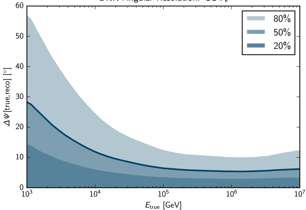
DNN Angular Resolution: CC \nu_e
