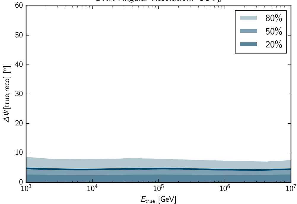
DNN Angular Resolution: CC \nu_\mu
