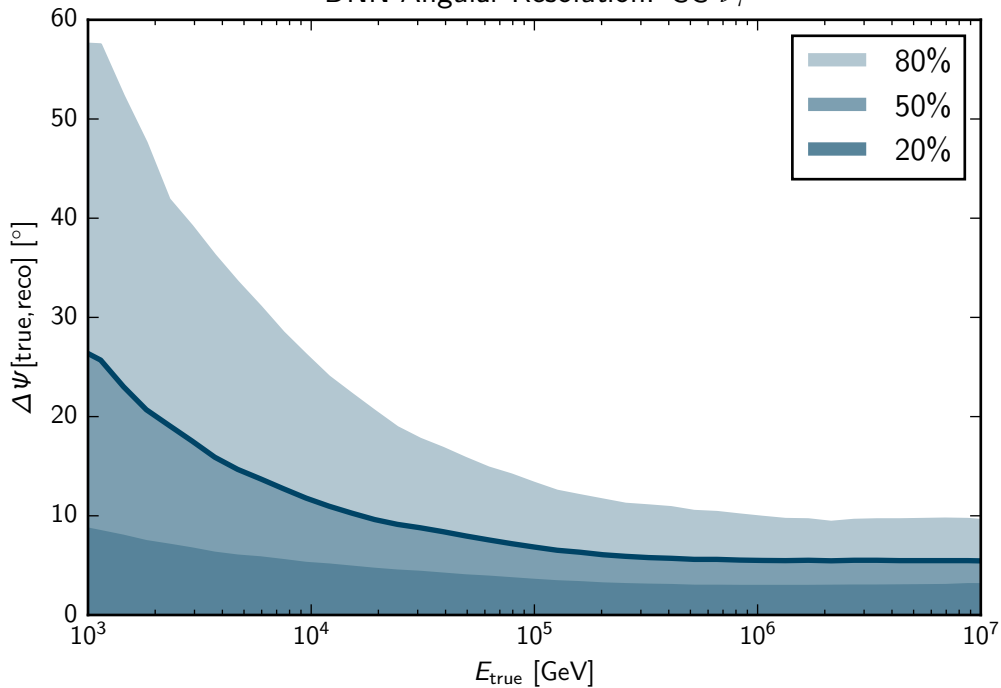
DNN Angular Resolution: CC \nu_\tau
