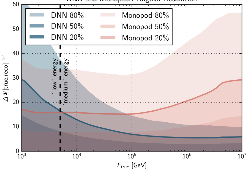
DNN and Monopod4 Angular Resolution
