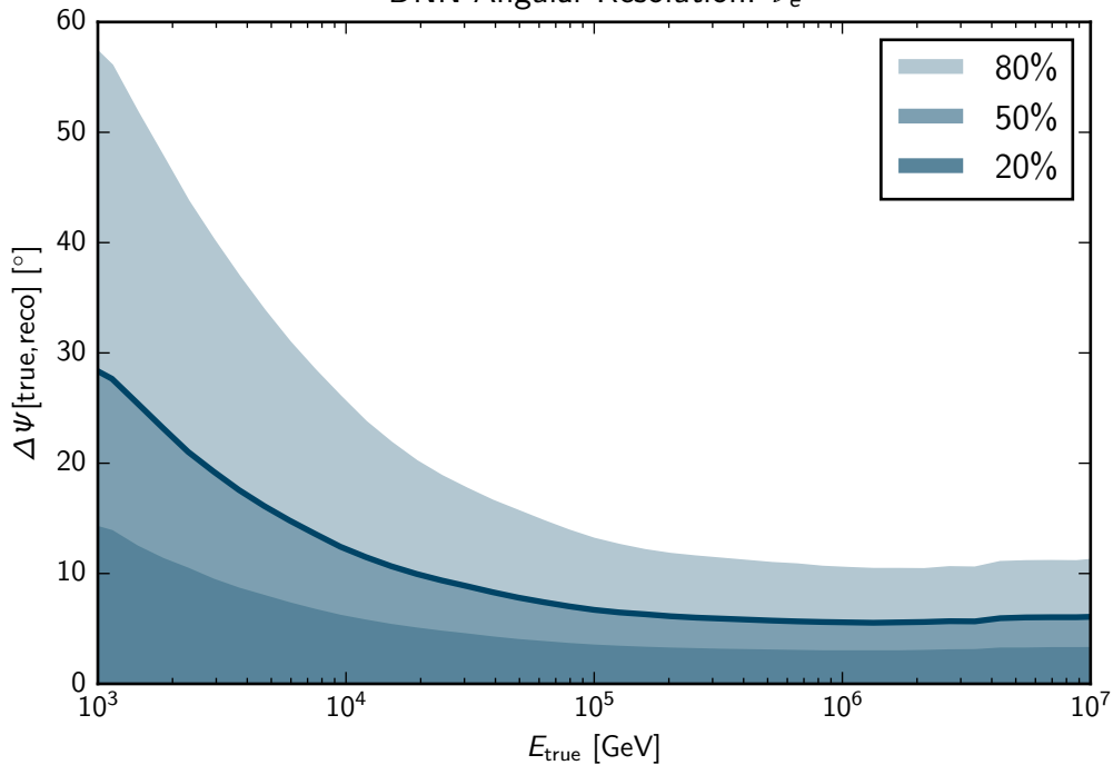
DNN Angular Resolution: \nu_e
