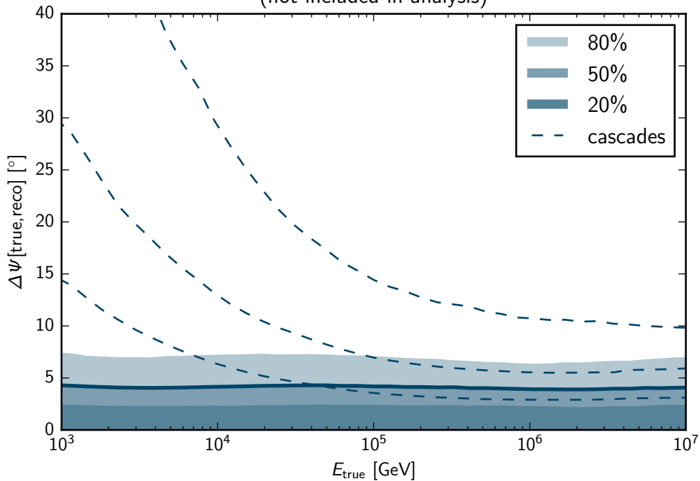
DNN Angular Resolution ( \nu_\mu and ID'd as track) (not included in analysis)
