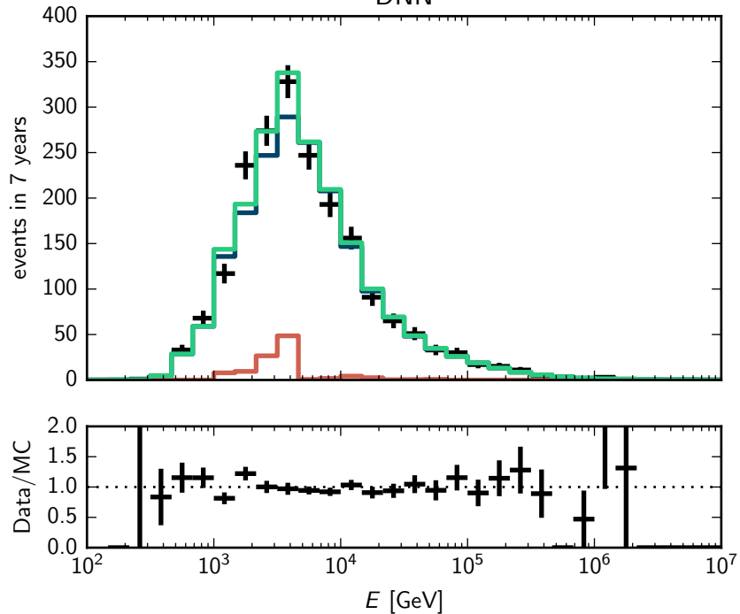
DNN
