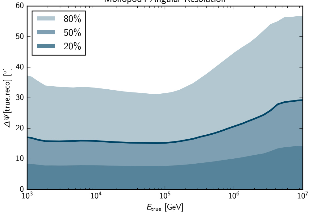
Monopod4 Angular Resolution
