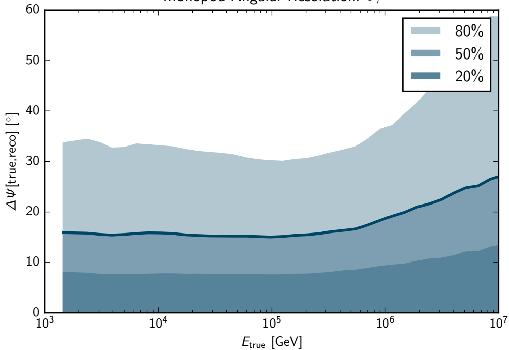
Monopod Angular Resolution: \nu_\tau
