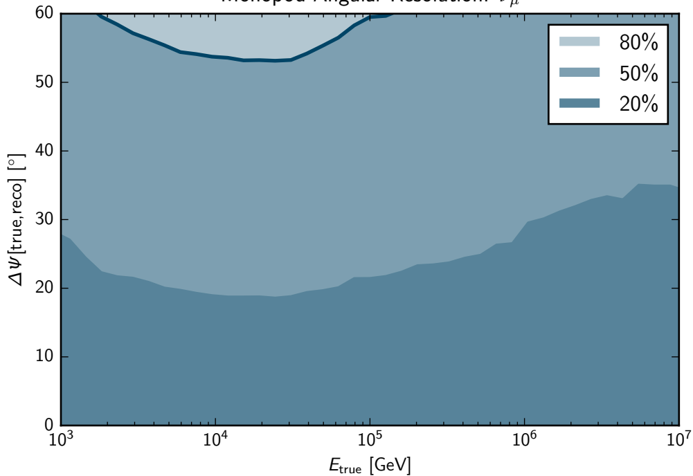
Monopod Angular Resolution: \nu_\mu
