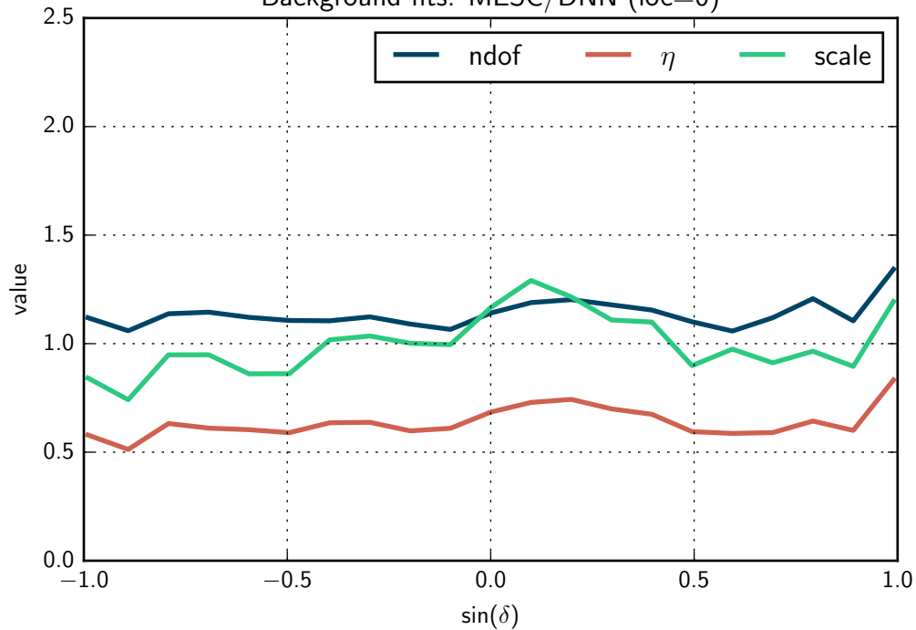
Background fits: MESC/DNN (loc=0)
