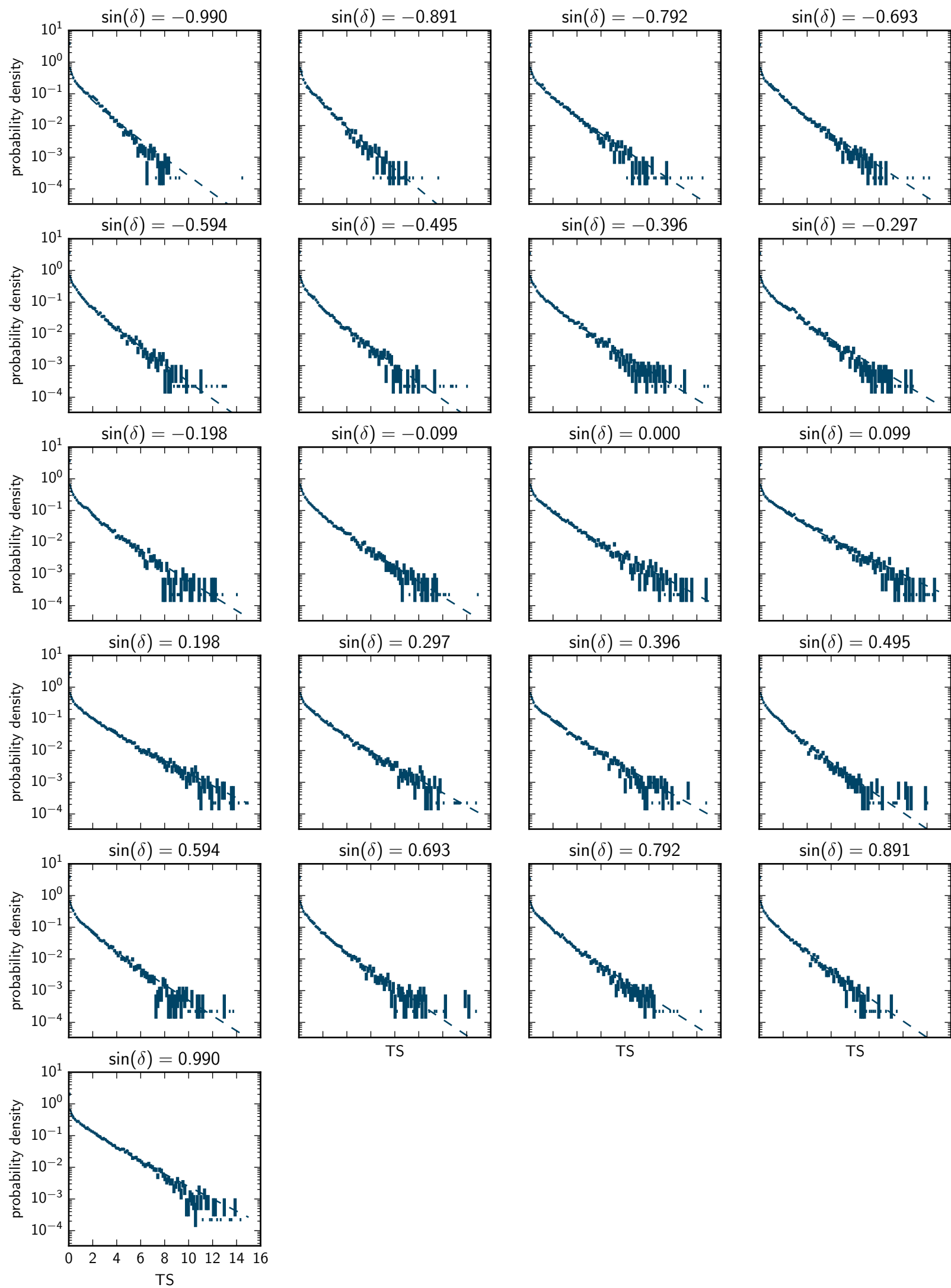
Background-only TS distributions: DNN (loc=0)
