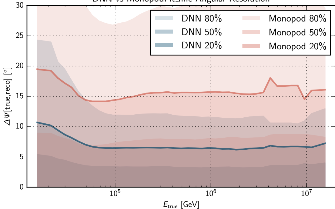
DNN vs MonopodFit_mie Angular Resolution
