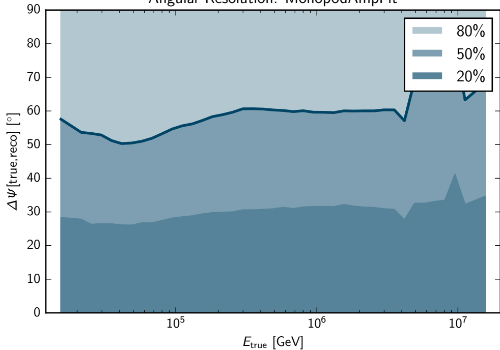
Angular Resolution: MonopodAmpFit
