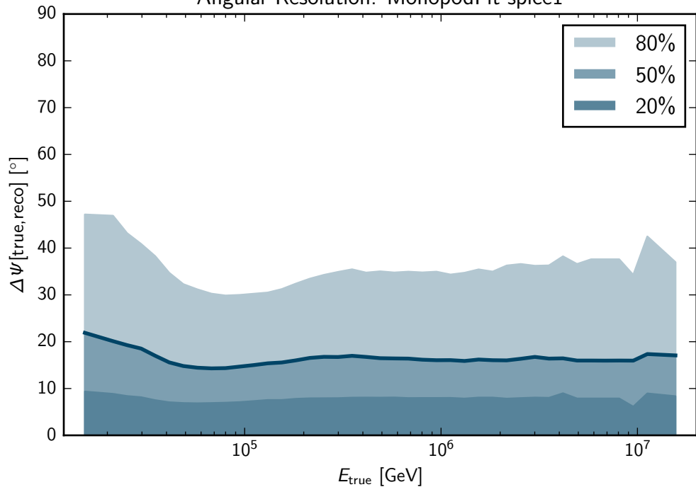
Angular Resolution: MonopodFit-spice1
