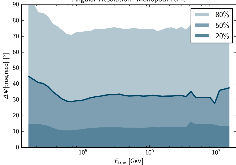
Angular Resolution: MonopodPreFit
