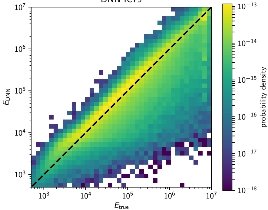
DNN IC79
